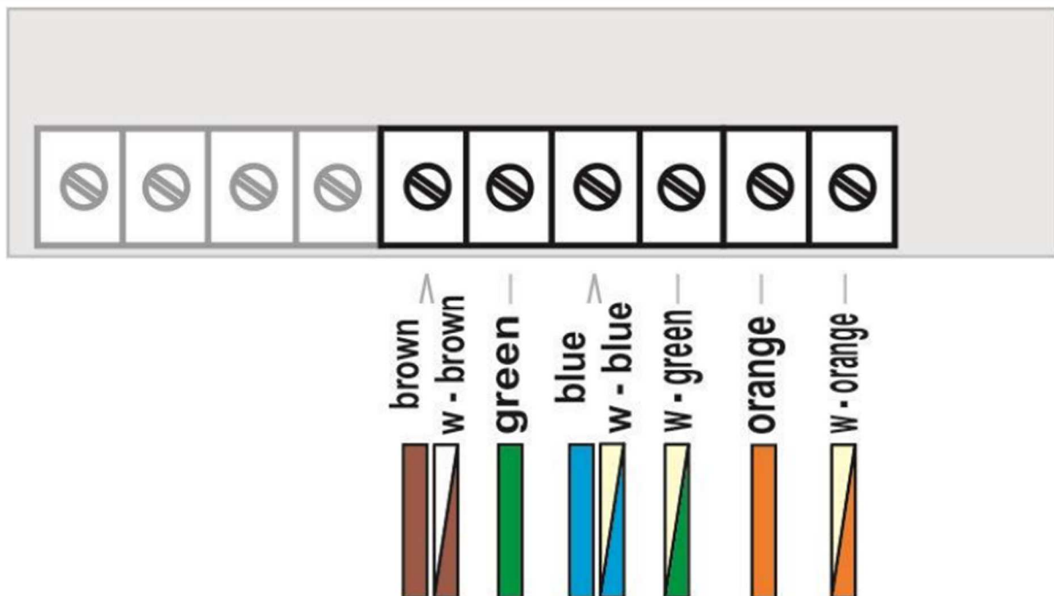
Figure 1 Terminal assignment PoE
